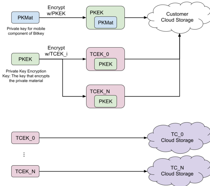
Figure 3: keys and data involved in Social Recovery setup.
